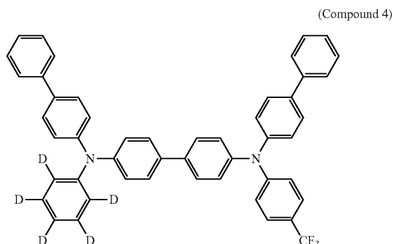
[Chemical Formula 20]
