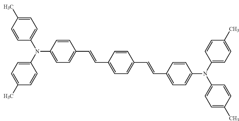
[Chemical Formula 69]
