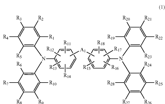
[Chemical Formula 1]
