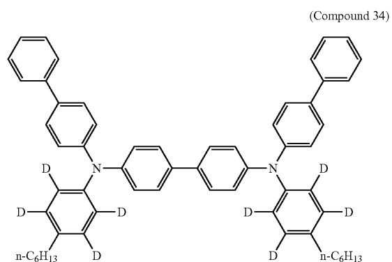
[Chemical Formula 48]
