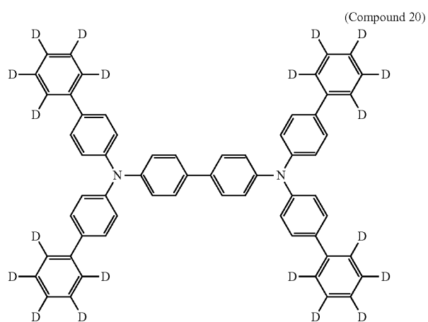
[Chemical Formula 34]
