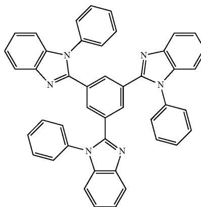
[Chemical Formula 64]
