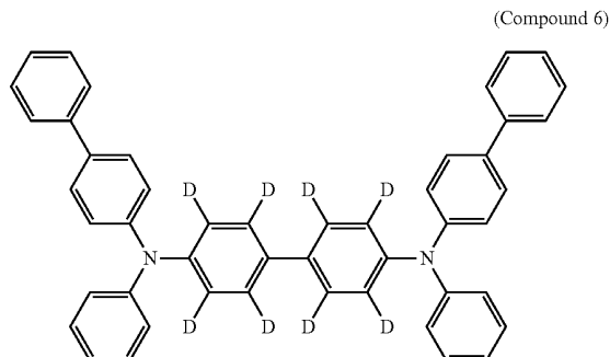
[Chemical Formula 20]
