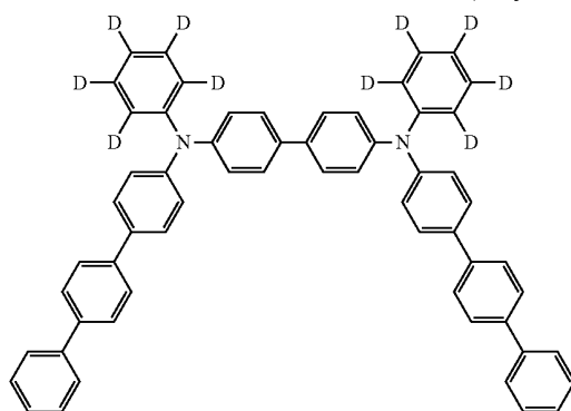
(Compound 12)
