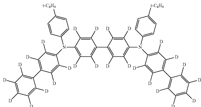
[Chemical Formula 31]
