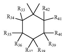
[Chemical Formula 9]
