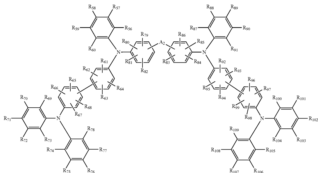
[Chemical Formula 7]
