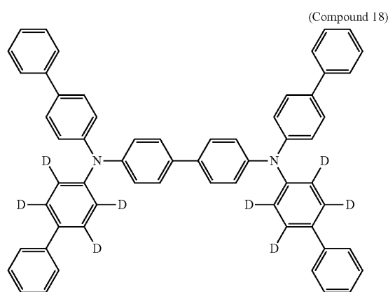
[Chemical Formula 32]
