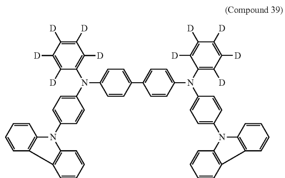
[Chemical Formula 53]
