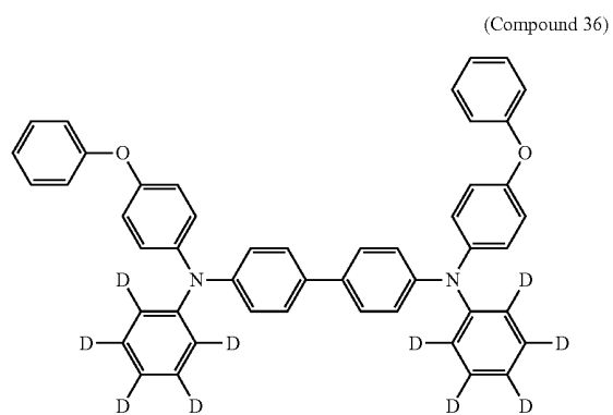
[Chemical Formula 50]
