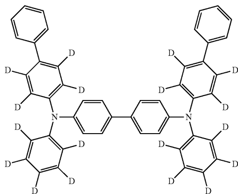
(Compound 7)
