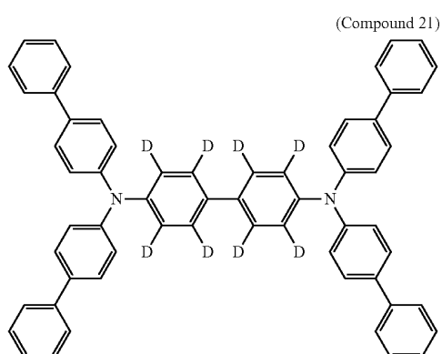
[Chemical Formula 35]
