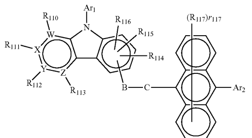
[Chemical Formula 16]
