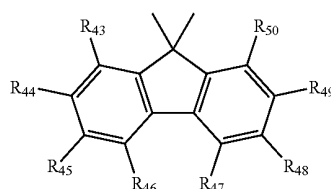
[Chemical Formula 4]
