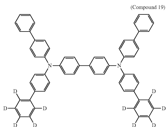
[Chemical Formula 33]
