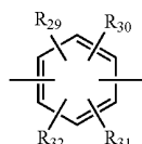
[Chemical Formula 8]
