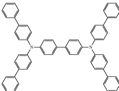
(Comparative Compound 51)
