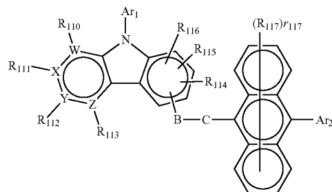
[Chemical Formula 16]
