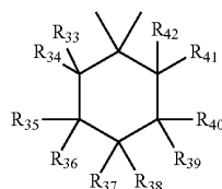
[Chemical Formula 3]
