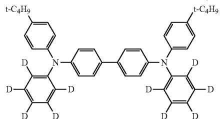
(Compound 11)
