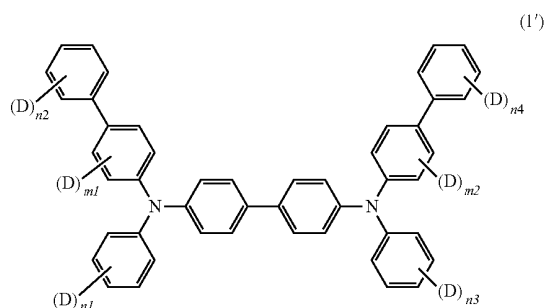
[Chemical Formula 13]
