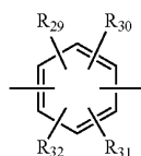
[Chemical Formula 8]
