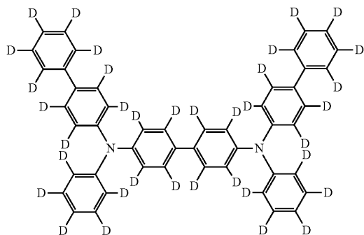
(Compound 9)
