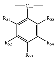
[Chemical Formula 12]
