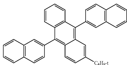
[Chemical Formula 69]
