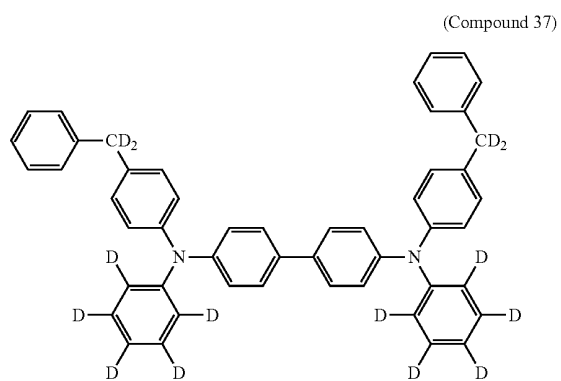
[Chemical Formula 51]
