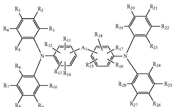
[Chemical Formula 1]
