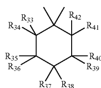
[Chemical Formula 3]
