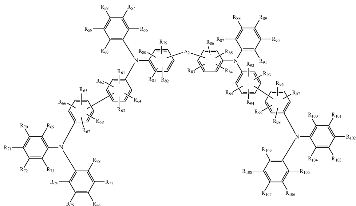
[Chemical Formula 7]
