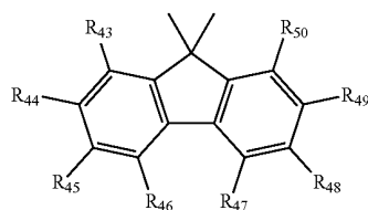
[Chemical Formula 10]
