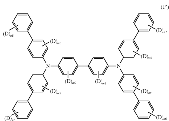
[Chemical Formula 14]
