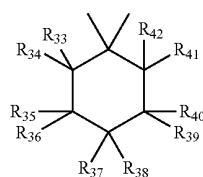
[Chemical Formula 9]
