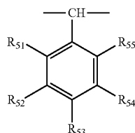
[Chemical Formula 6]
