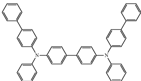
(Comparative Compound 50)
