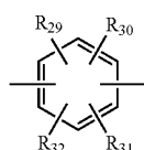
[Chemical Formula 2]
