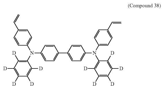
[Chemical Formula 52]
