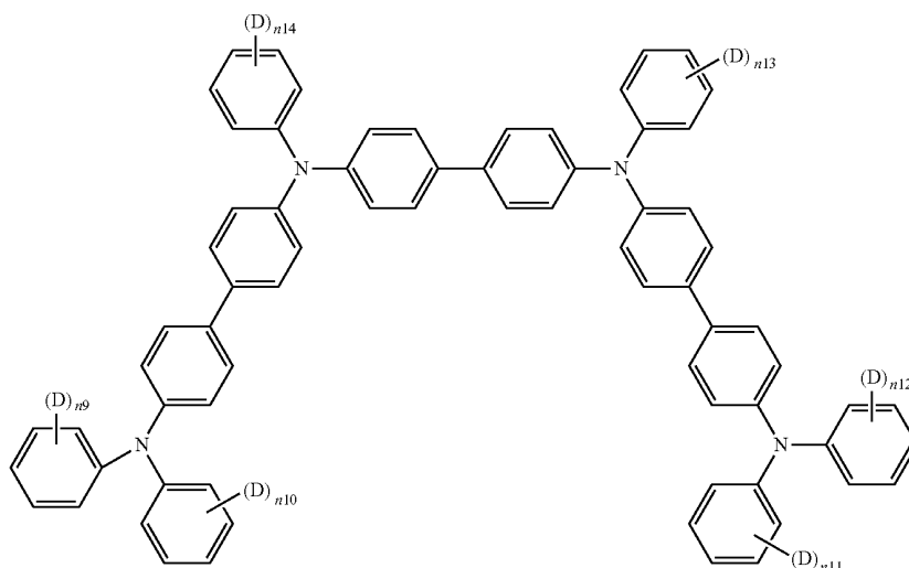
[Chemical Formula 15]
