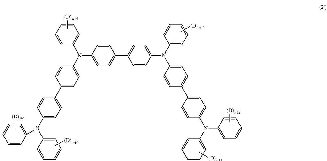
[Chemical Formula 15]
