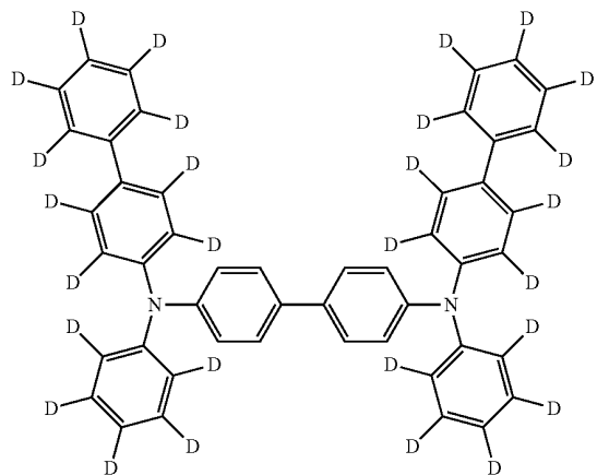
(Compound 8)
