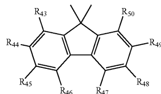
[Chemical Formula 10]
